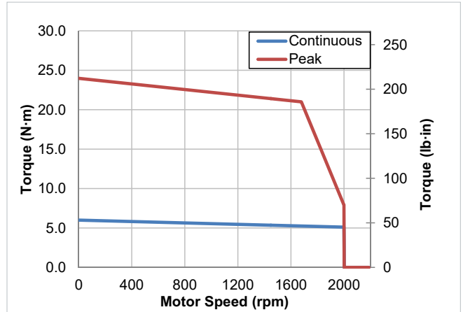
S-180-44-B Torque vs Speed
