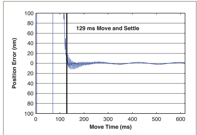
ANT130V-5-PLUS step and settle performance at 75 mm/s, with a settle spec of \pm 20 nm, and a step size of 5 mm. Outstanding settling time enhances throughput of most applications.
