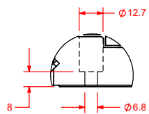
DETAIL A SCALE 2 : 5 MOUNTING HOLES TYP.
