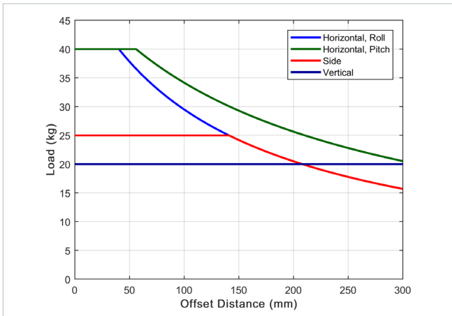
Cantilevered load capability of ATX165SL(E)-150.
