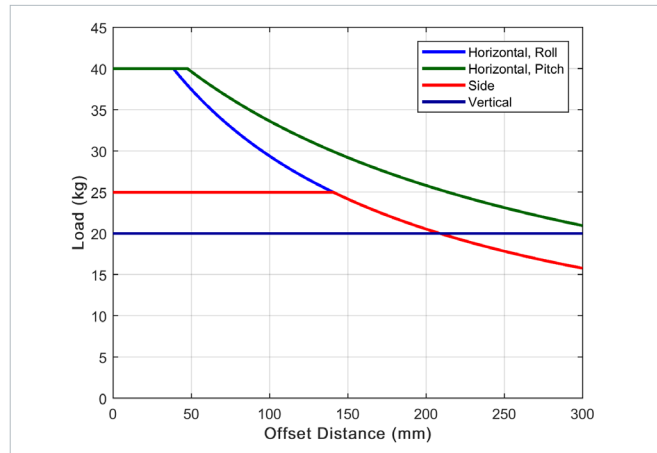
Cantilevered load capability of ATX165SL(E)-200.
