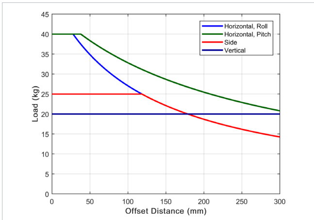
Cantilevered load capability of ATX165SL(E)-250.
