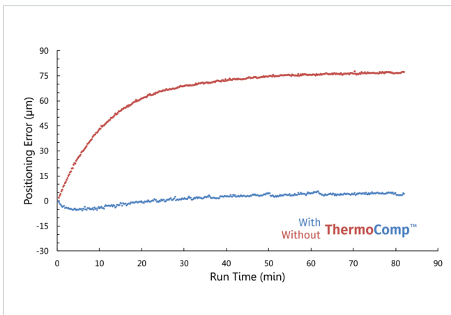
Measurement data showing successful compensation of internal heating-related positioning errors during prolonged operation of a ball screw stage using the ThermoComp feature. Results are typical of ball screw stage performance with and without ThermoComp.
