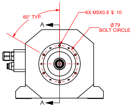
STAGE REAR, REAR COVER REMOVED BOLT PATTERN FOR WET-CUT ACCESSORY MOUNTING
