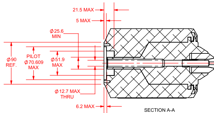
SECTION A-A ENVELOPE LIMITS FOR WET-CUT ACCESSORY
