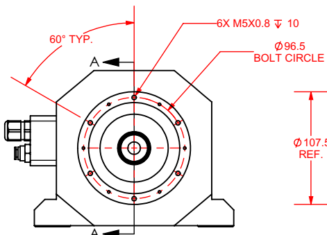
STAGE REAR, REAR COVER REMOVED BOLT PATTERN FOR WET-CUT ACCESSORY MOUNTING
